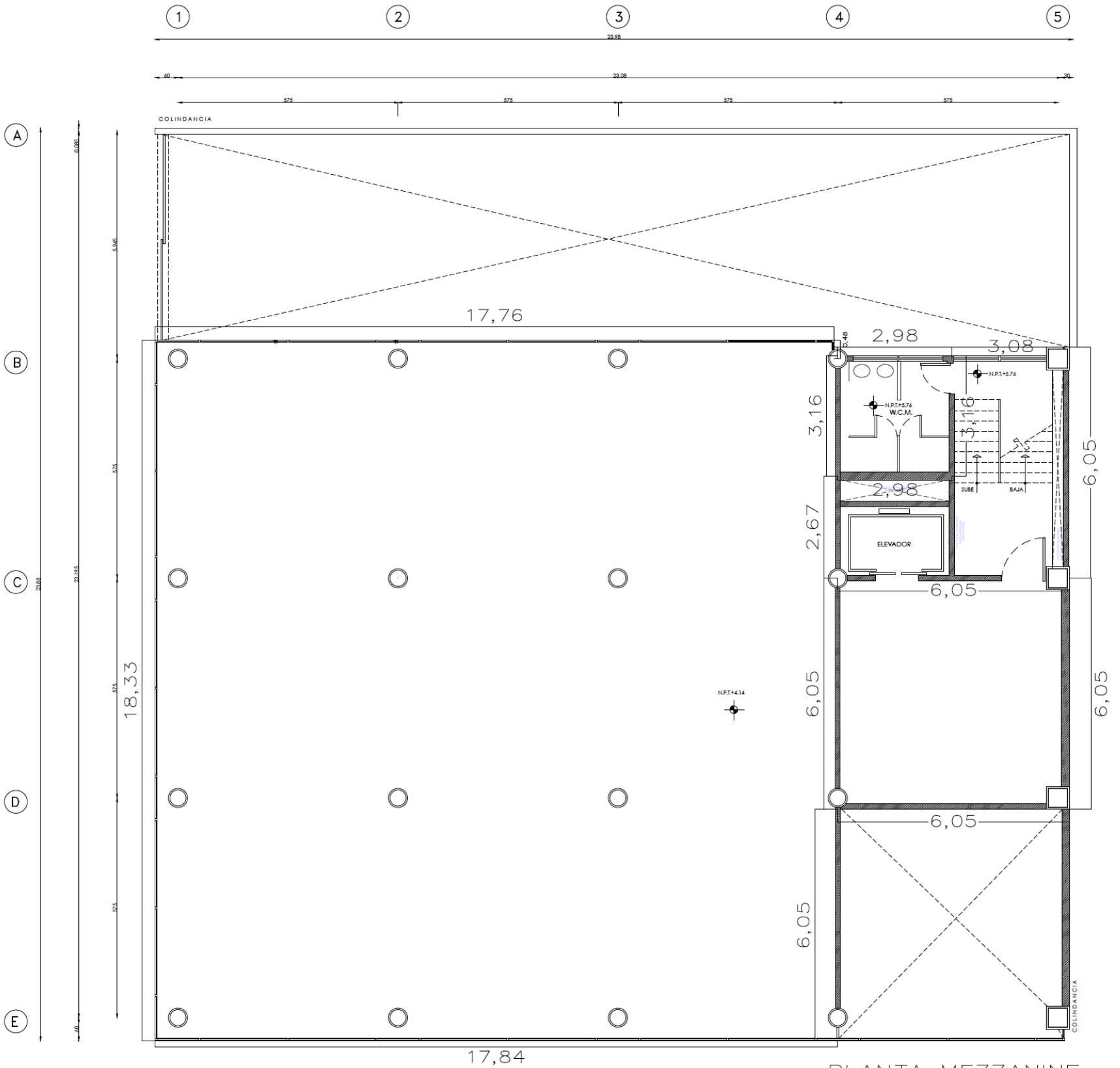
PLANTA MEZZANINE
